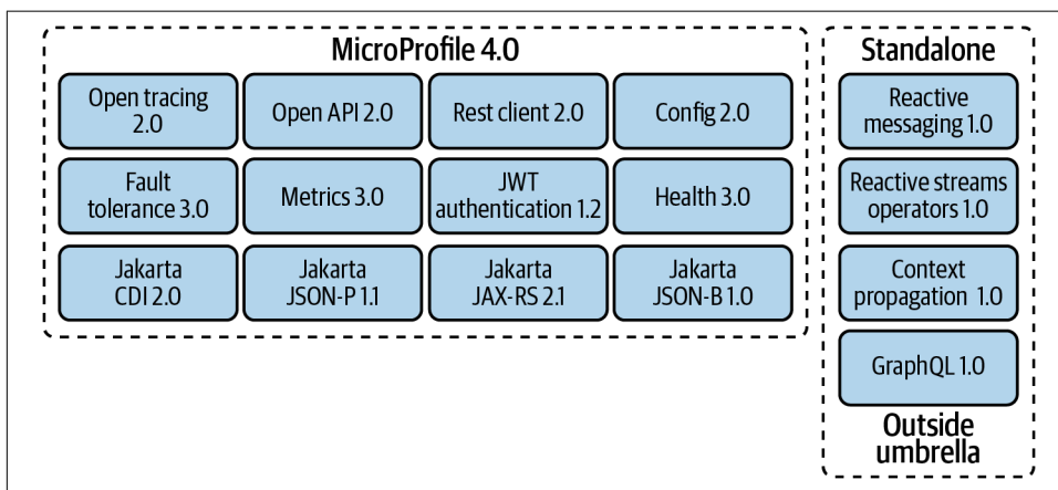
Figure 5-3. MicroProfile technologies overview
