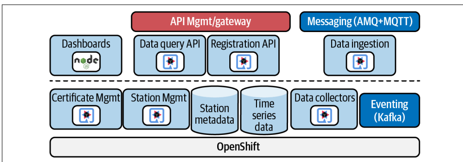
Figure 7-4. Quarkus for IoT project architecture
